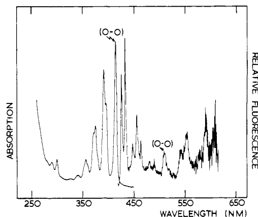
Figure 3. Absorption and fluorescence spectra of all-trans -1,3,5,7,9,11,13-tetradecaheptaene in 77 K EPA. Absorption obtained with a 2 nm band-pass. Fluorescence excited at 405.4 nm and detected with 1 nm resolution through a Schott KV-418 filter.
